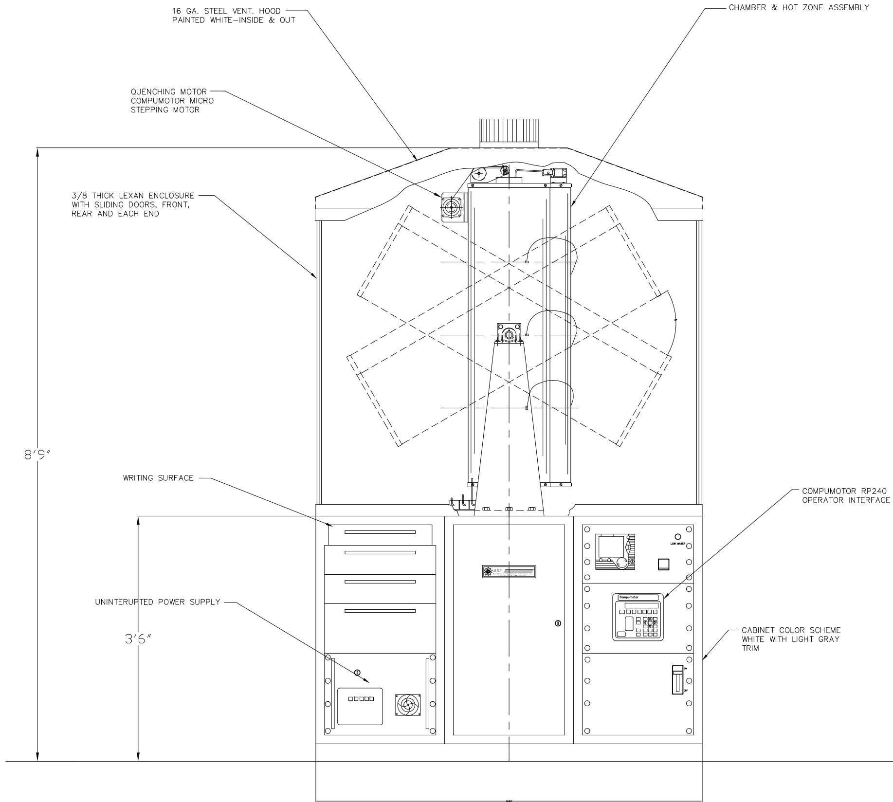
FRONT ELEVATION
