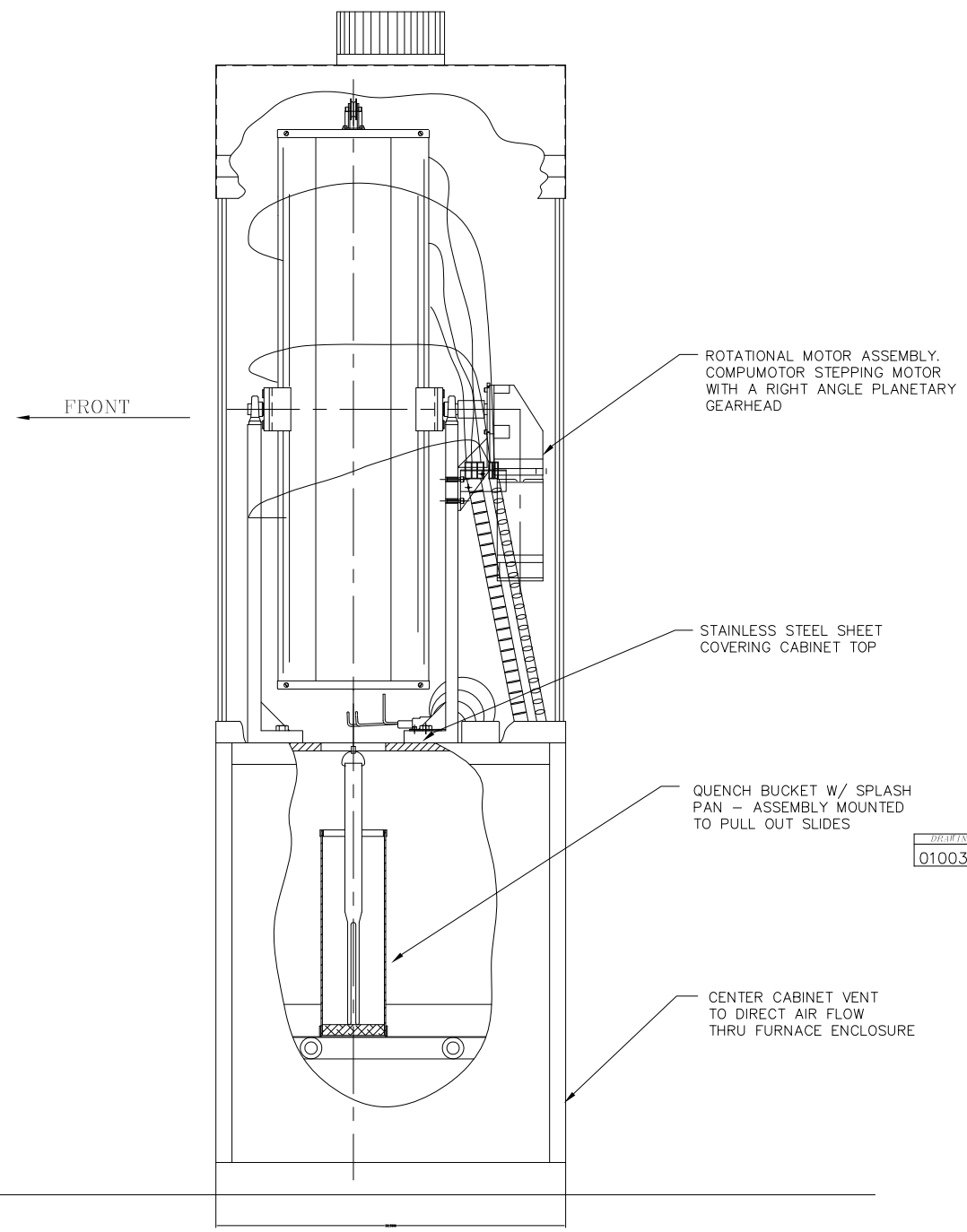
SIDE VIEW
